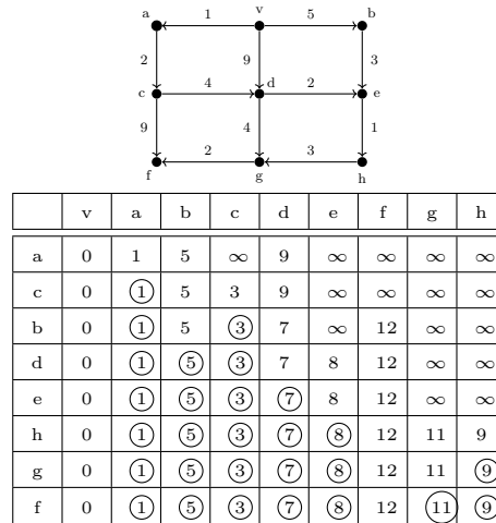
Figure: An example of the single-source shortest-paths algorithm. Source: redrawn from [Manber 1989, Figure 7.18].
